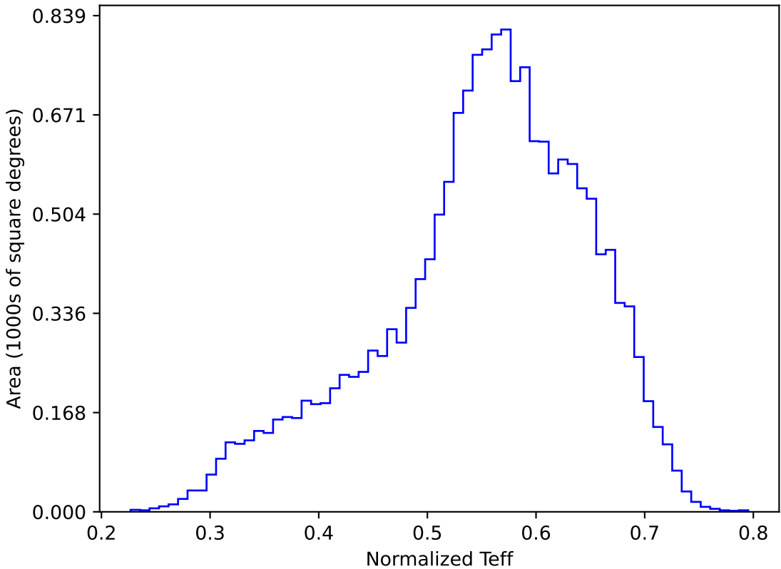
too_elab_r32_d2_griz_v3.4_10yrs WFD y band: Normalized Teff
