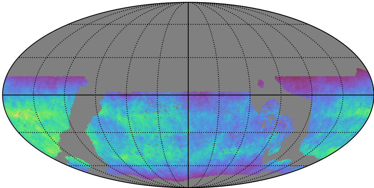
too_elab_r32_d2_griz_v3.4_10yrs WFD u band: Normalized Teff
