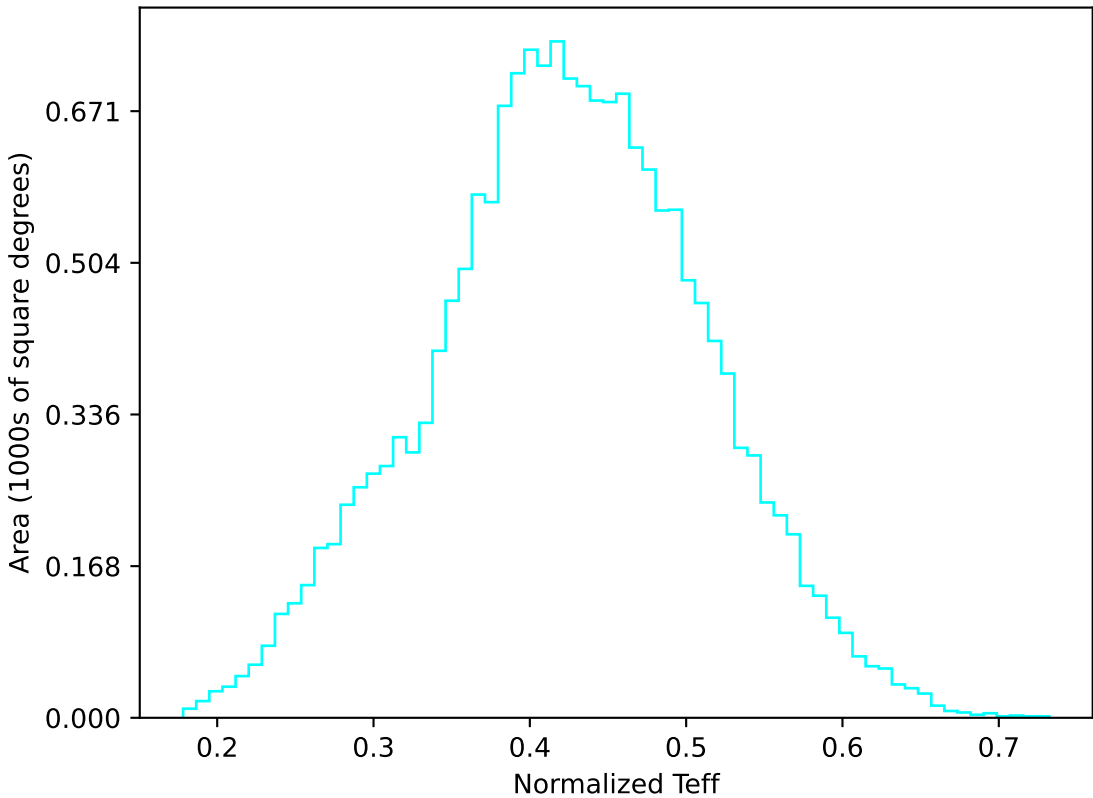
too_elab_r32_d2_griz_v3.4_10yrs WFD u band: Normalized Teff
