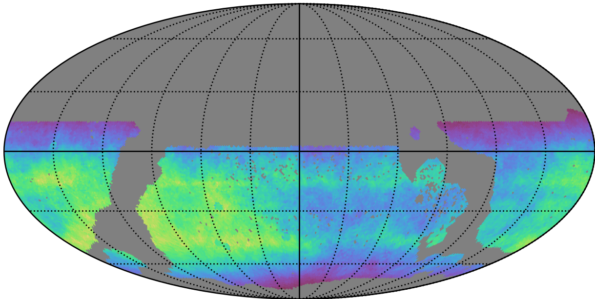
too_elab_r32_d2_griz_v3.4_10yrs WFD i band: Normalized Teff
