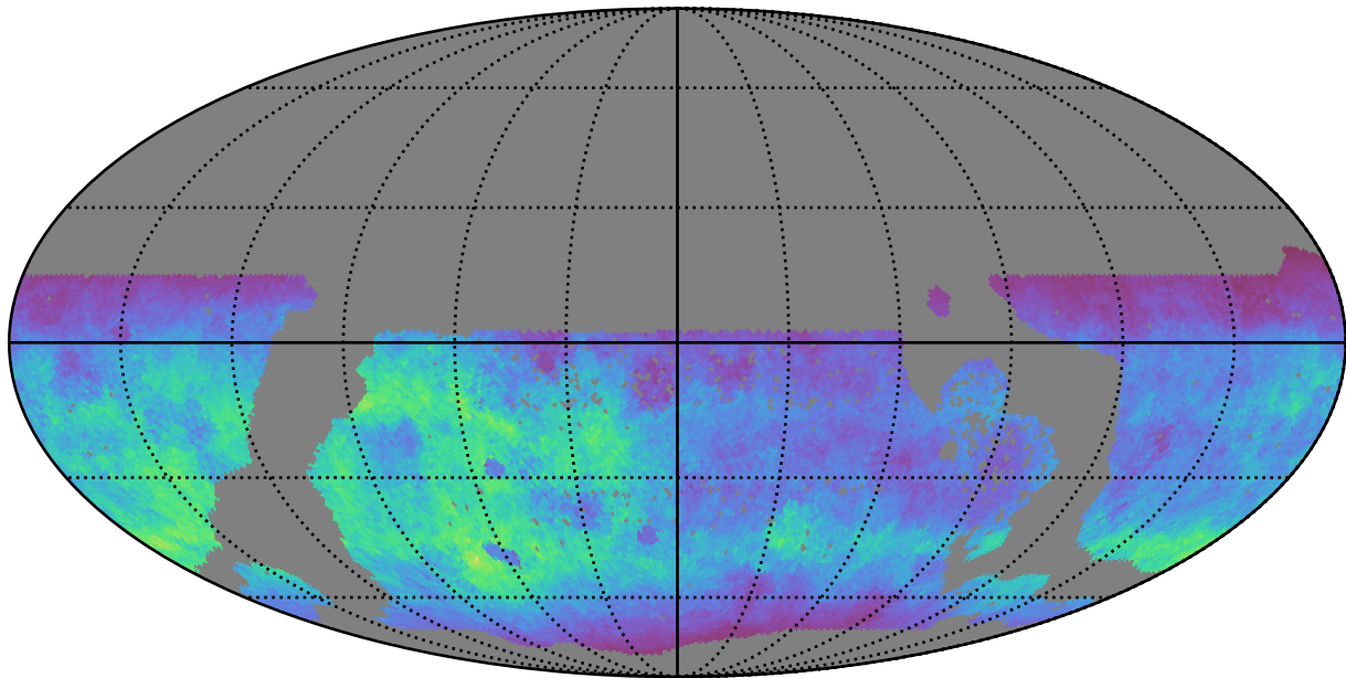
too_elab_r32_d2_griz_v3.4_10yrs WFD g band: Normalized Teff
