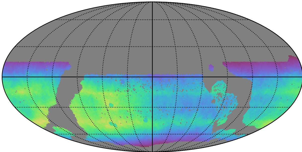
too_elab_r32_d2_griz_v3.4_10yrs WFD all bands: Normalized Teff
