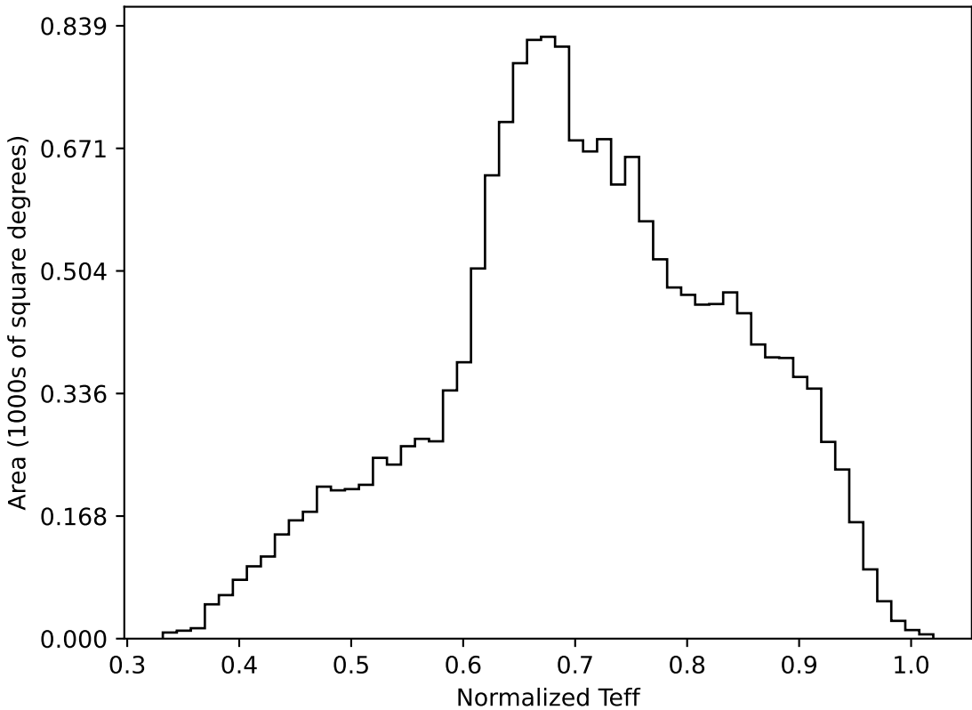
too_elab_r32_d2_griz_v3.4_10yrs WFD all bands: Normalized Teff
