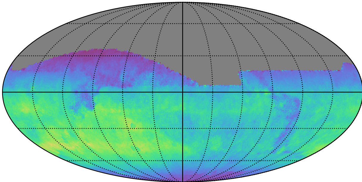
too_elab_r32_d2_griz_v3.4_10yrs All sky z band: Normalized Teff
