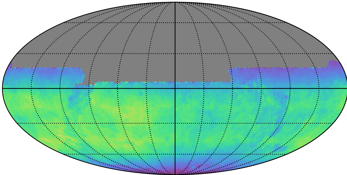
too_elab_r32_d2_griz_v3.4_10yrs All sky y band: Normalized Teff
