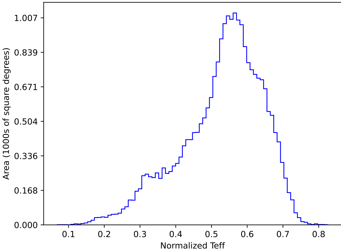
too_elab_r32_d2_griz_v3.4_10yrs All sky y band: Normalized Teff
