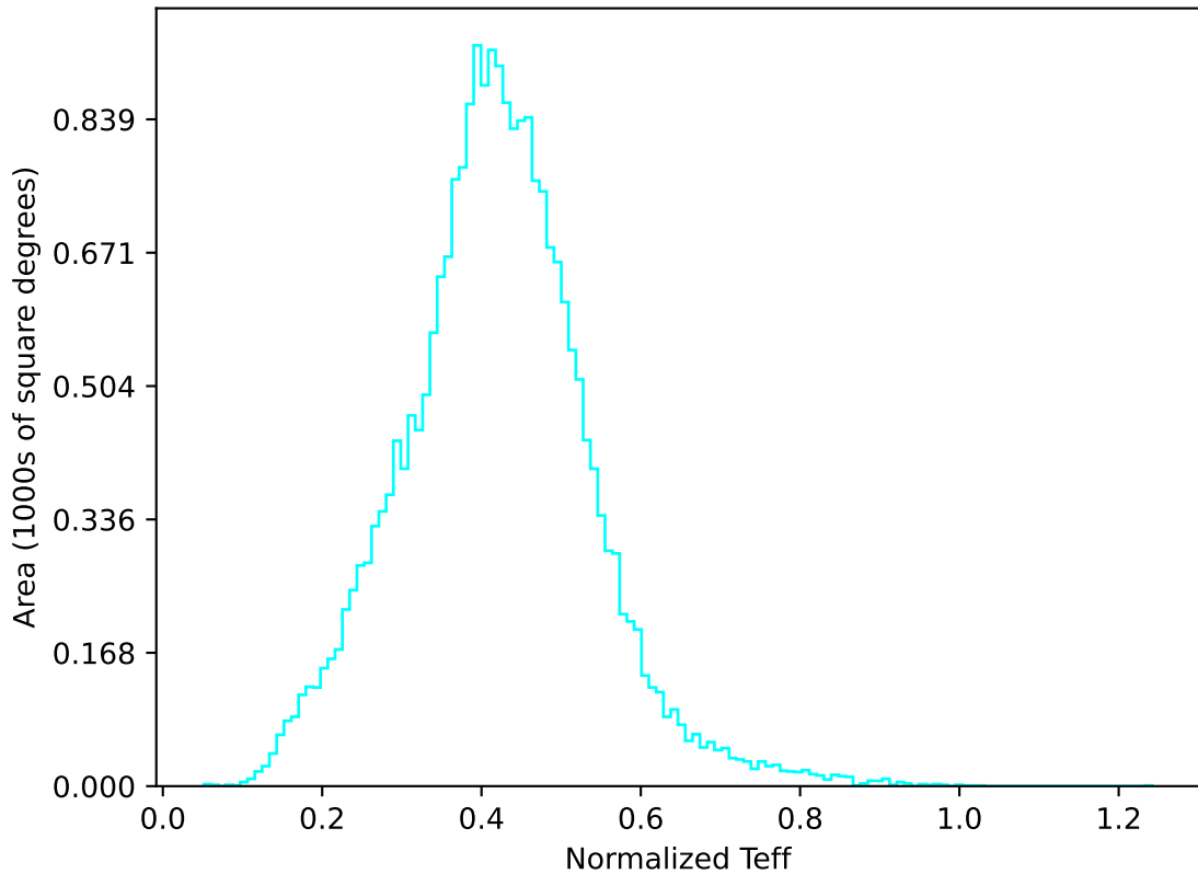
too_elab_r32_d2_griz_v3.4_10yrs All sky u band: Normalized Teff
