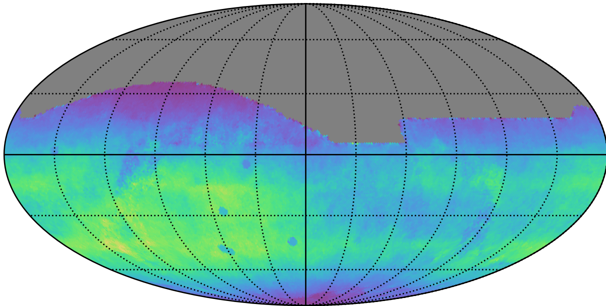
too_elab_r32_d2_griz_v3.4_10yrs All sky r band: Normalized Teff
