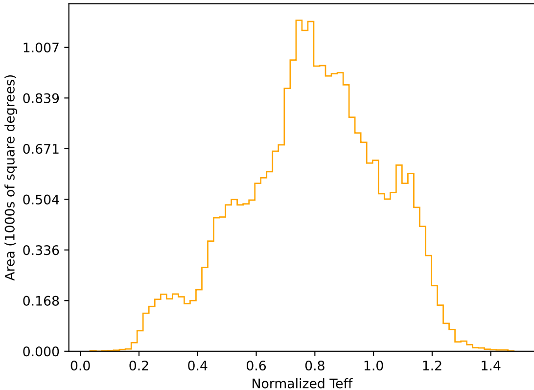
too_elab_r32_d2_griz_v3.4_10yrs All sky r band: Normalized Teff
