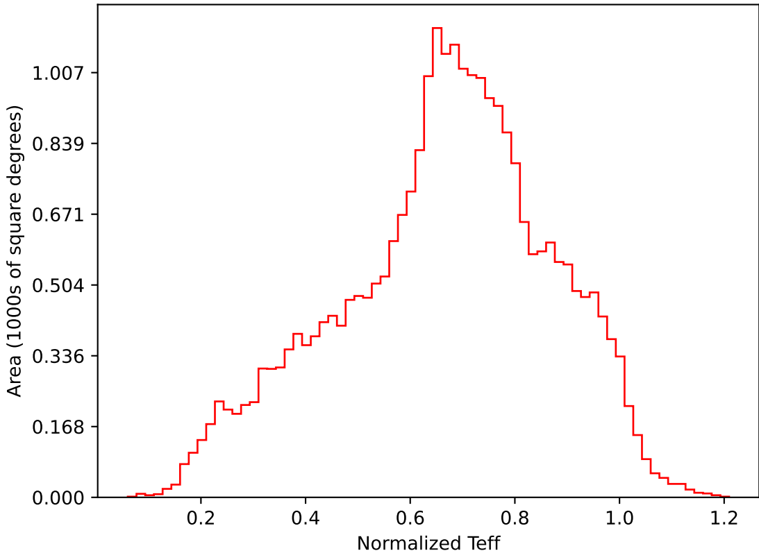
too_elab_r32_d2_griz_v3.4_10yrs All sky i band: Normalized Teff
