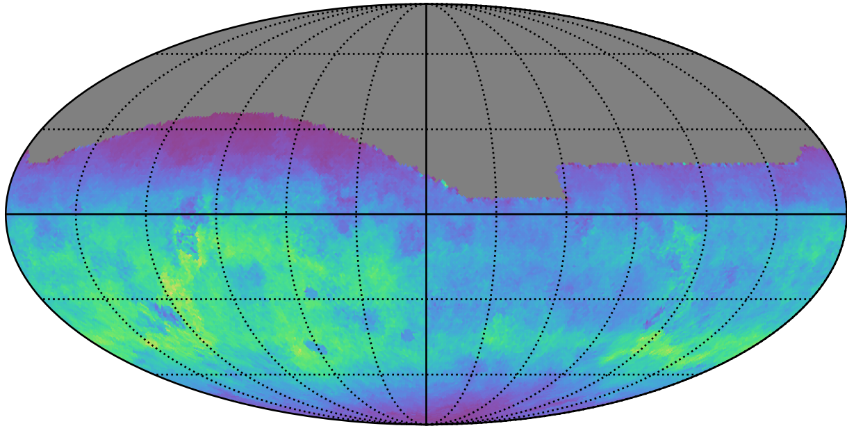
too_elab_r32_d2_griz_v3.4_10yrs All sky g band: Normalized Teff
