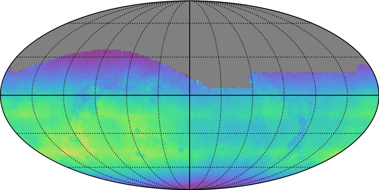
too_elab_r32_d2_griz_v3.4_10yrs All sky all bands: Normalized Teff
