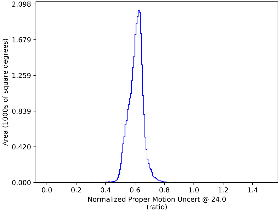
too_elab_r32_d2_griz_v3.4_10yrs All sky: Normalized Proper Motion Uncert @ 24.0
