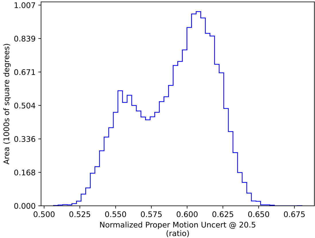
too_elab_r32_d2_griz_v3.4_10yrs WFD: Normalized Proper Motion Uncert @ 20.5
