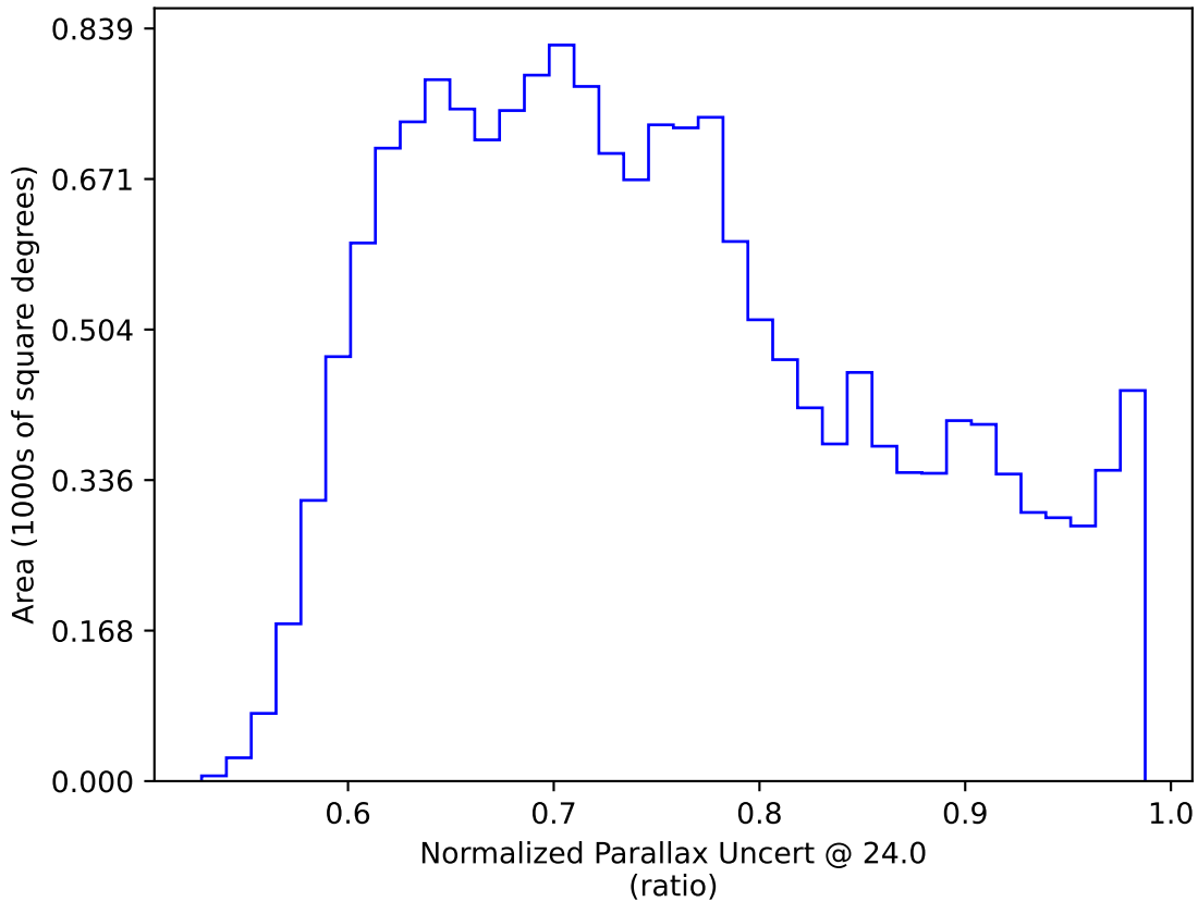
too_elab_r32_d2_griz_v3.4_10yrs WFD: Normalized Parallax Uncert @ 24.0
