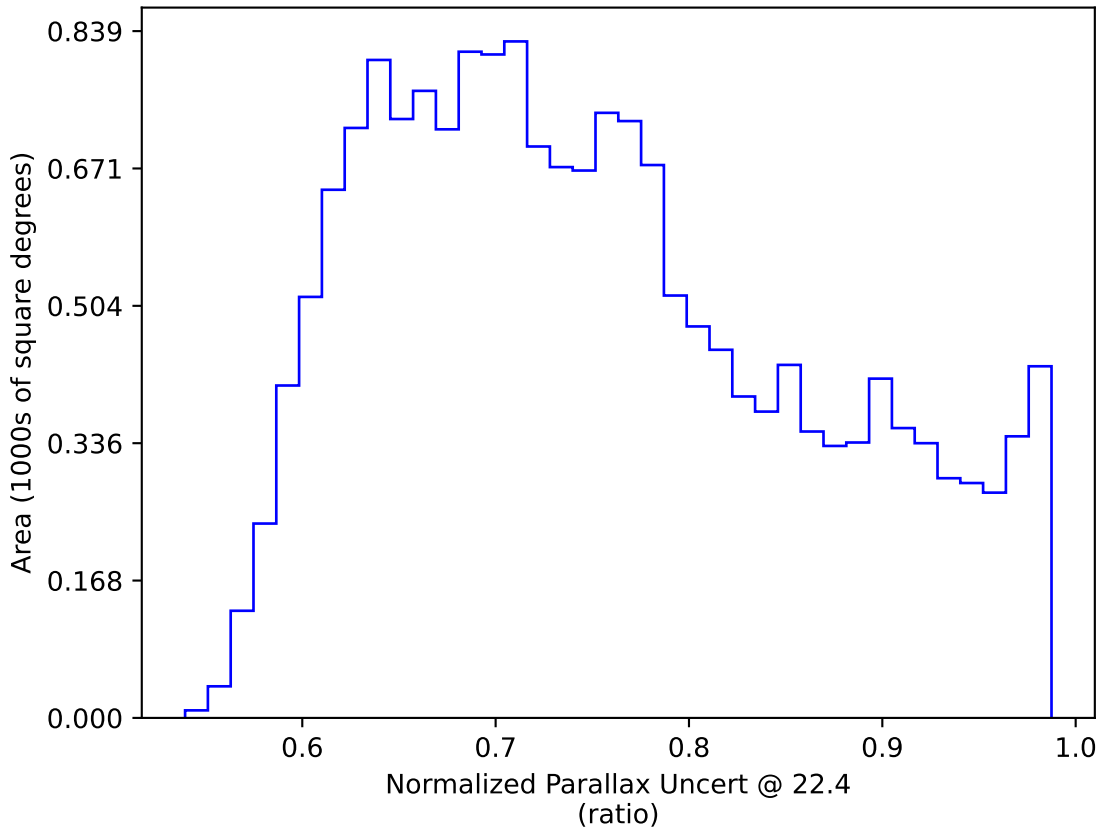
too_elab_r32_d2_griz_v3.4_10yrs WFD: Normalized Parallax Uncert @ 22.4
