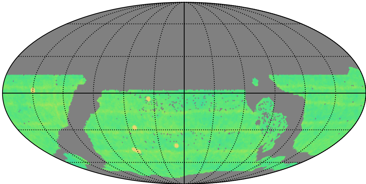
too_elab_r32_d2_griz_v3.4_10yrs WFD all bands: N Unique Nights
