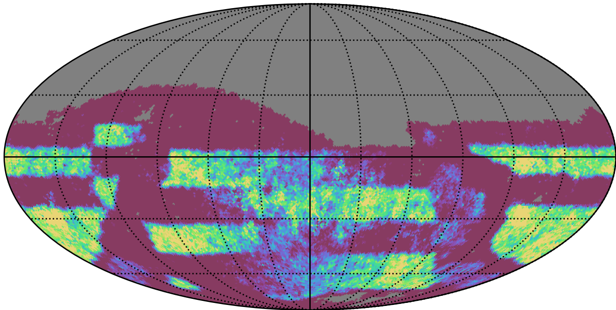
too_elab_r32_d2_griz_v3.4_10yrs Yr 3-4 z band: NVisits
