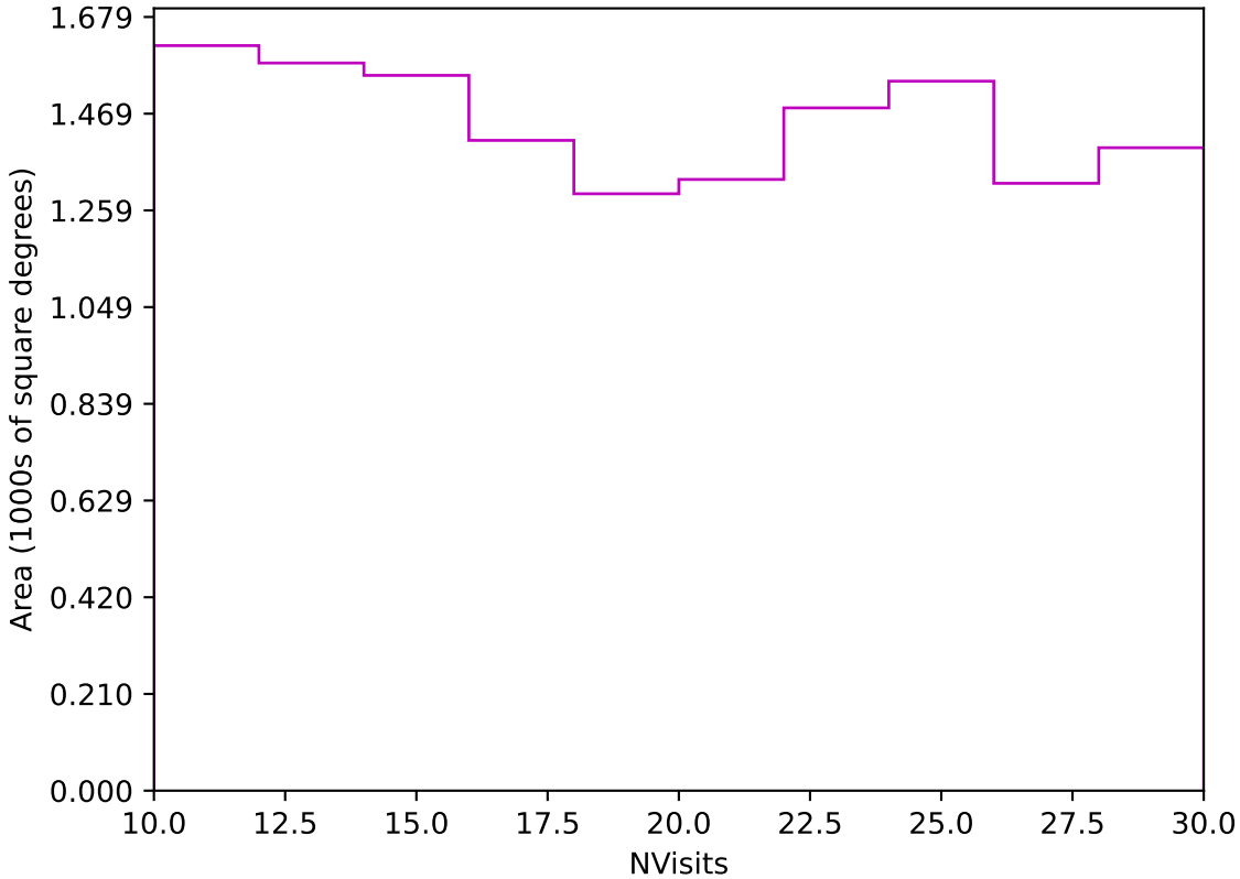
too_elab_r32_d2_griz_v3.4_10yrs Yr 3-4 z band: NVisits
