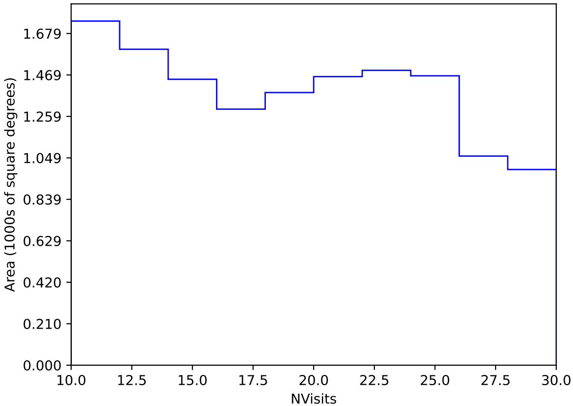
too_elab_r32_d2_griz_v3.4_10yrs Yr 3-4 y band: NVisits
