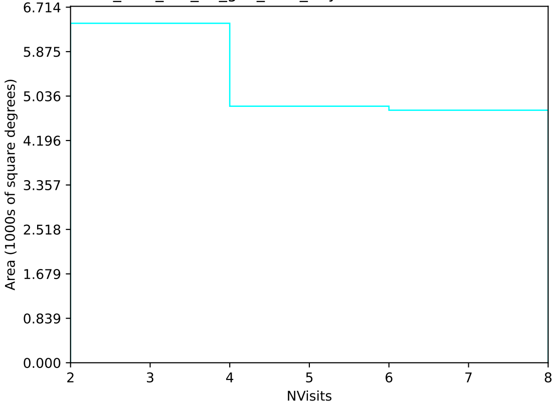
too_elab_r32_d2_griz_v3.4_10yrs Yr 3-4 u band: NVisits
