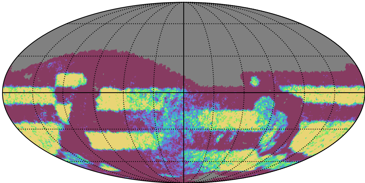
too_elab_r32_d2_griz_v3.4_10yrs Yr 3-4 r band: NVisits
