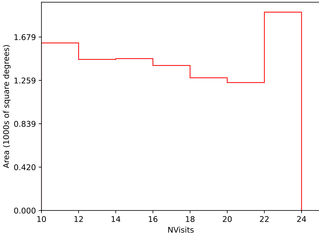
too_elab_r32_d2_griz_v3.4_10yrs Yr 3-4 i band: NVisits
