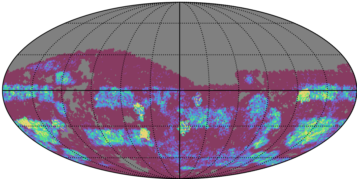
too_elab_r32_d2_griz_v3.4_10yrs Yr 3-4 g band: NVisits
