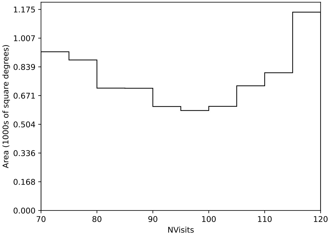
too_elab_r32_d2_griz_v3.4_10yrs Yr 3-4 all bands: NVisits
