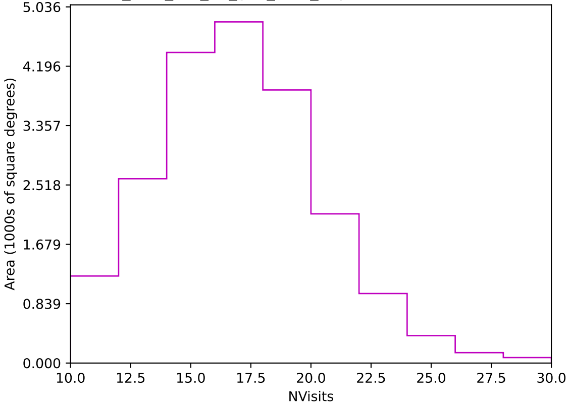
too_elab_r32_d2_griz_v3.4_10yrs Yr 1 z band: NVisits
