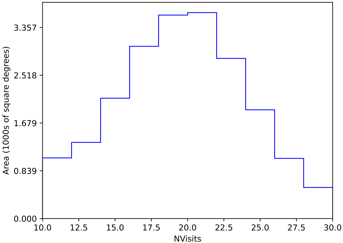
too_elab_r32_d2_griz_v3.4_10yrs Yr 1 y band: NVisits
