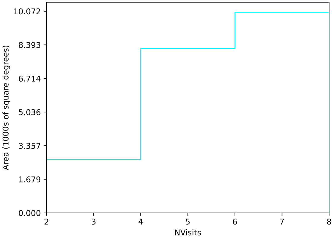
too_elab_r32_d2_griz_v3.4_10yrs Yr 1 u band: NVisits
