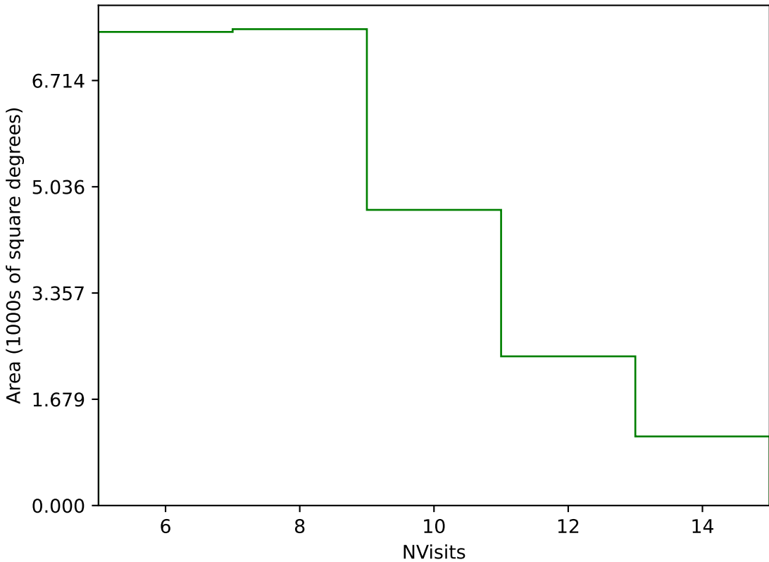
too_elab_r32_d2_griz_v3.4_10yrs Yr 1 g band: NVisits
