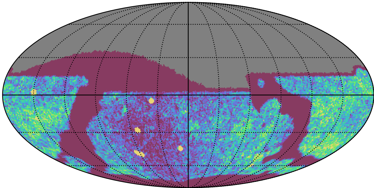
too_elab_r32_d2_griz_v3.4_10yrs Yr 1 all bands: NVisits
