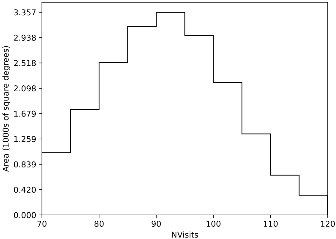
too_elab_r32_d2_griz_v3.4_10yrs Yr 1 all bands: NVisits
