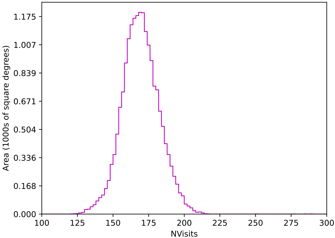
too_elab_r32_d2_griz_v3.4_10yrs WFD z band: NVisits
