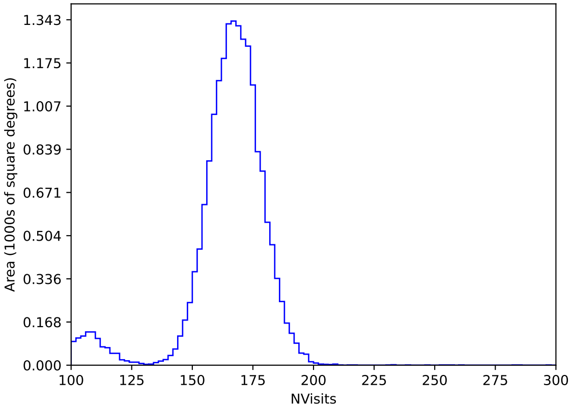
too_elab_r32_d2_griz_v3.4_10yrs WFD y band: NVisits
