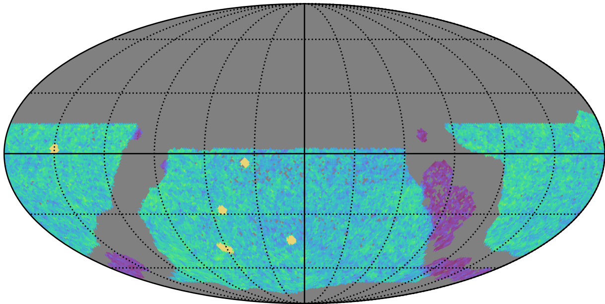
too_elab_r32_d2_griz_v3.4_10yrs WFD u band: NVisits
