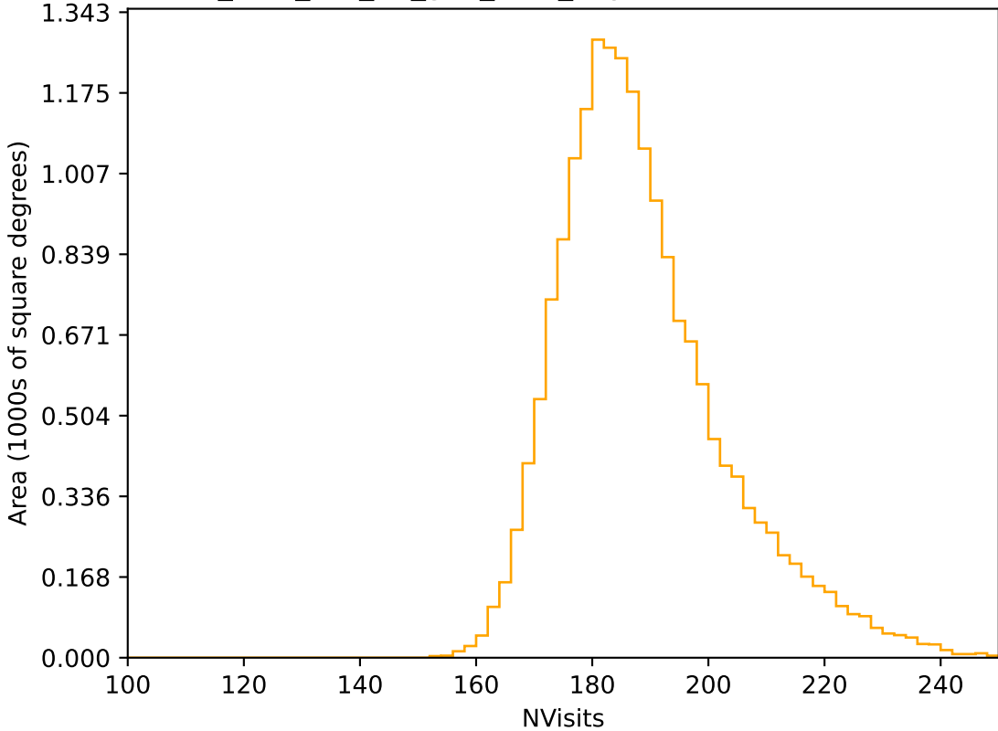
too_elab_r32_d2_griz_v3.4_10yrs WFD r band: NVisits
