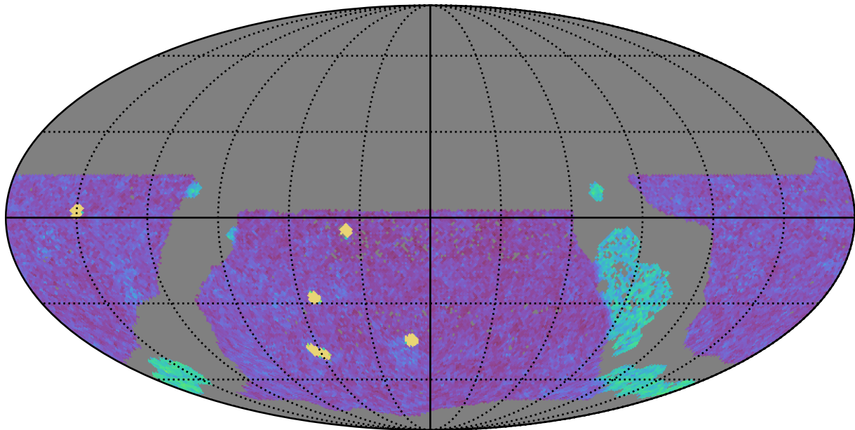
too_elab_r32_d2_griz_v3.4_10yrs WFD g band: NVisits
