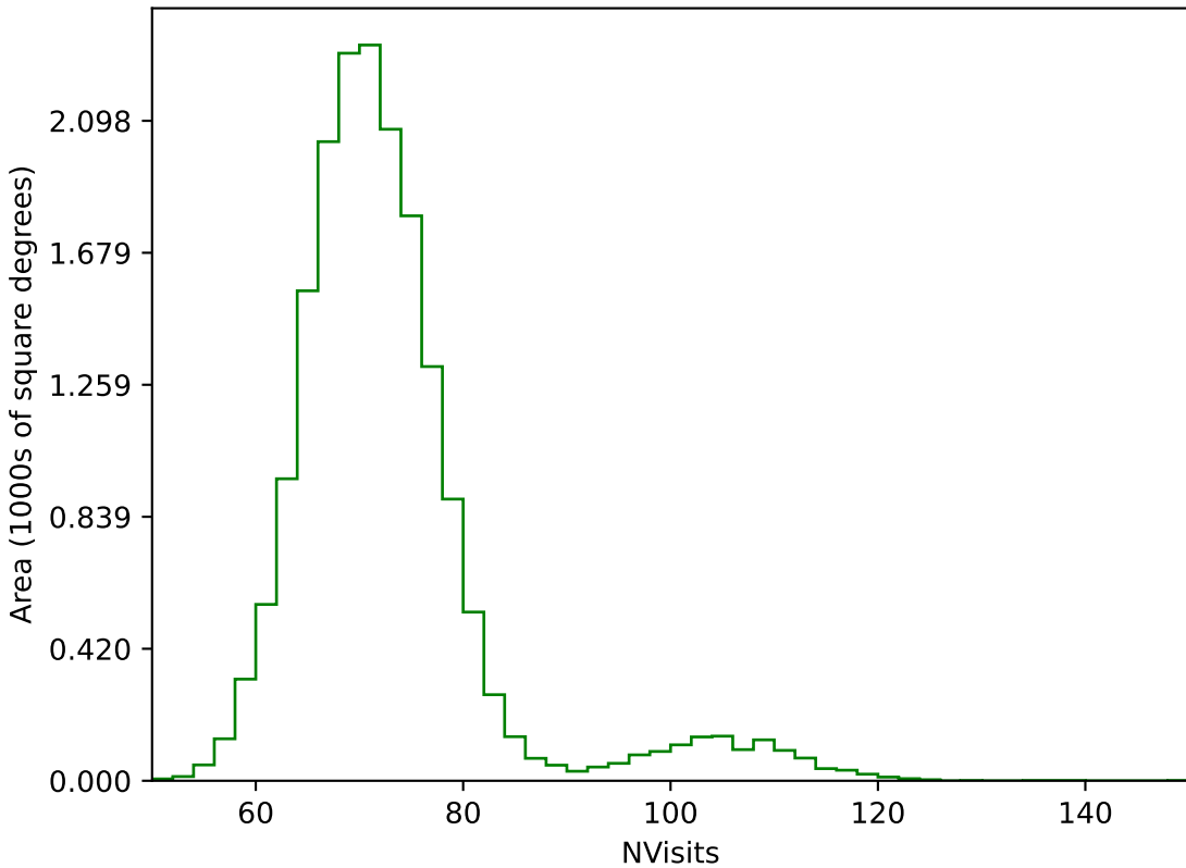
too_elab_r32_d2_griz_v3.4_10yrs WFD g band: NVisits
