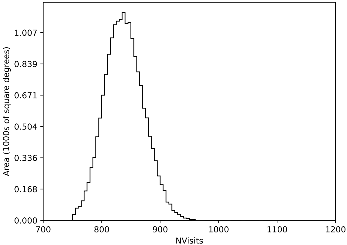
too_elab_r32_d2_griz_v3.4_10yrs WFD all bands: NVisits
