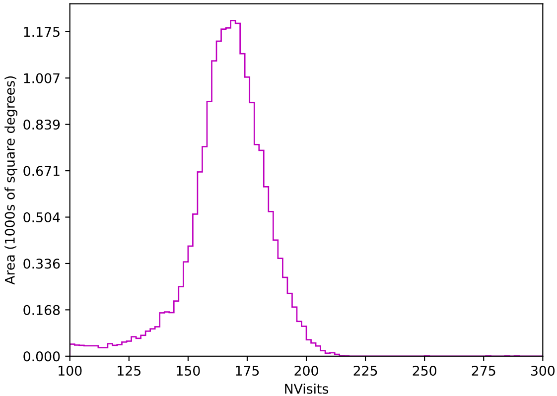
too_elab_r32_d2_griz_v3.4_10yrs All sky z band: NVisits
