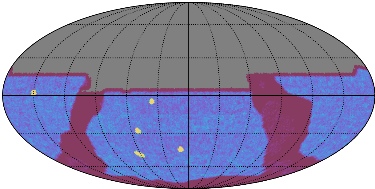
too_elab_r32_d2_griz_v3.4_10yrs All sky y band: NVisits
