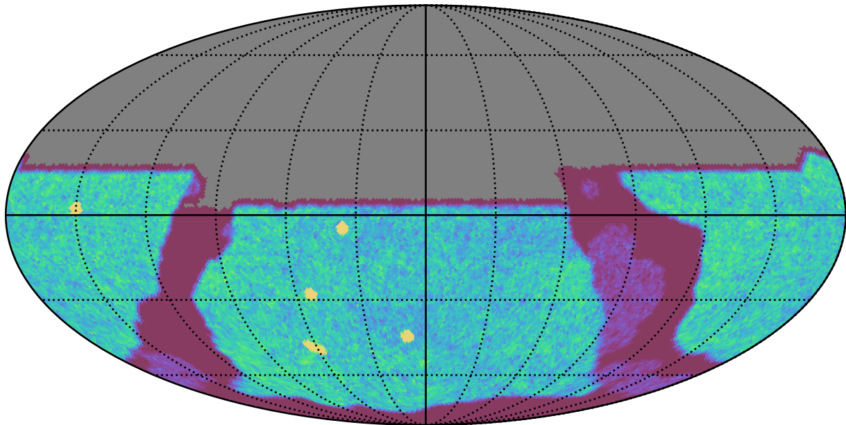
too_elab_r32_d2_griz_v3.4_10yrs All sky u band: NVisits
