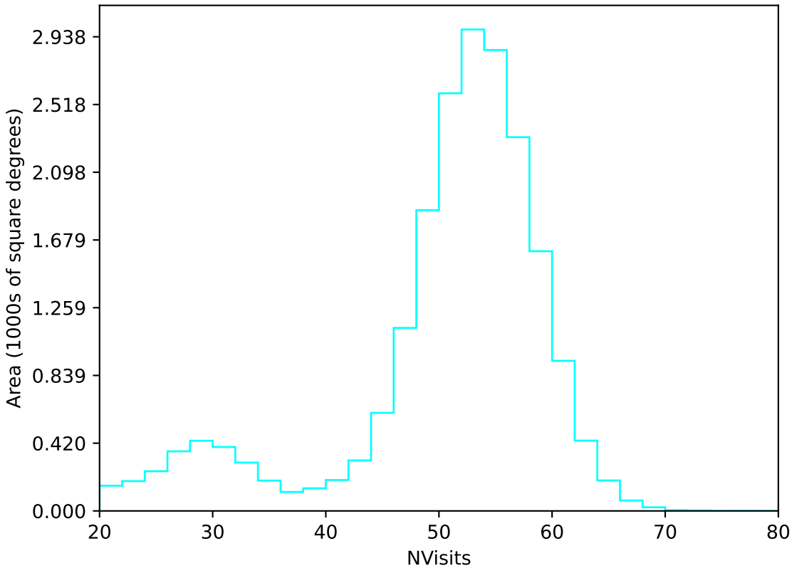
too_elab_r32_d2_griz_v3.4_10yrs All sky u band: NVisits
