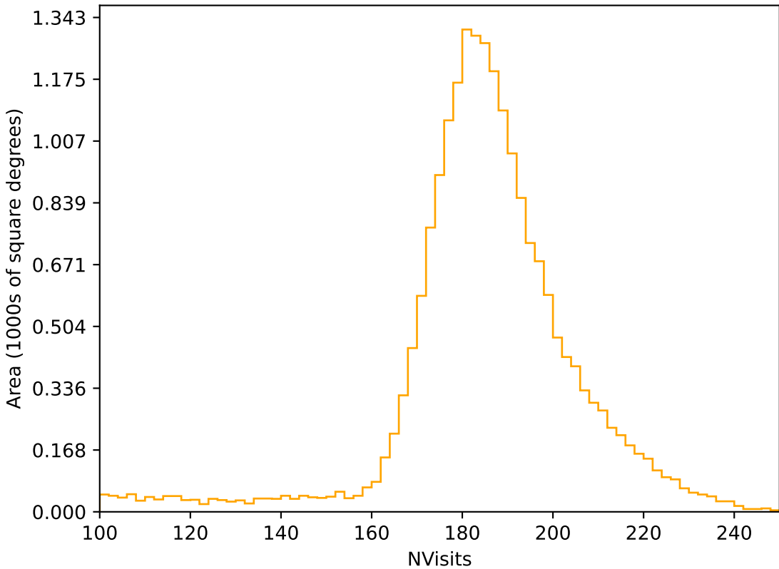
too_elab_r32_d2_griz_v3.4_10yrs All sky r band: NVisits
