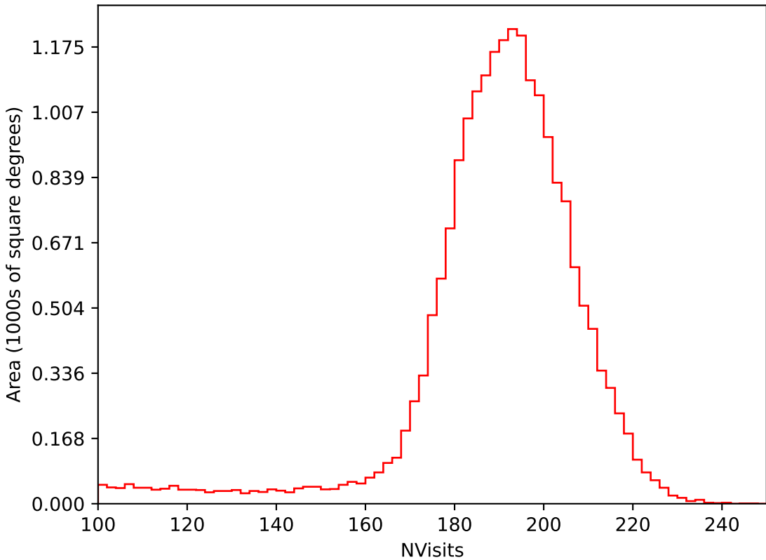
too_elab_r32_d2_griz_v3.4_10yrs All sky i band: NVisits
