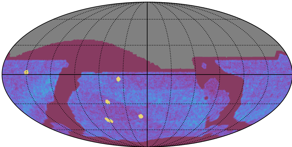
too_elab_r32_d2_griz_v3.4_10yrs All sky all bands: NVisits
