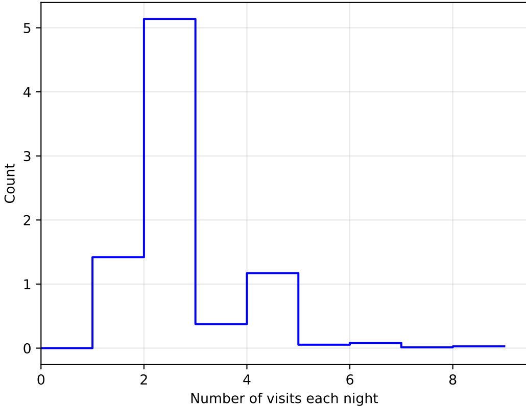
too_elab_r32_d2_griz_v3.4_10yrs WFD: NVisitsPerNight
